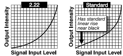
FIGURE 3-9 GAMMA CURVE
