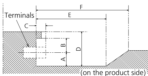
Sectional view of terminal b
