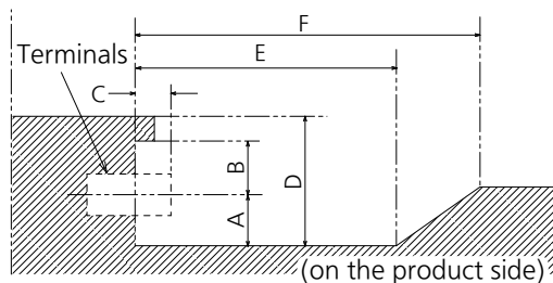
Sectional view of terminal b
