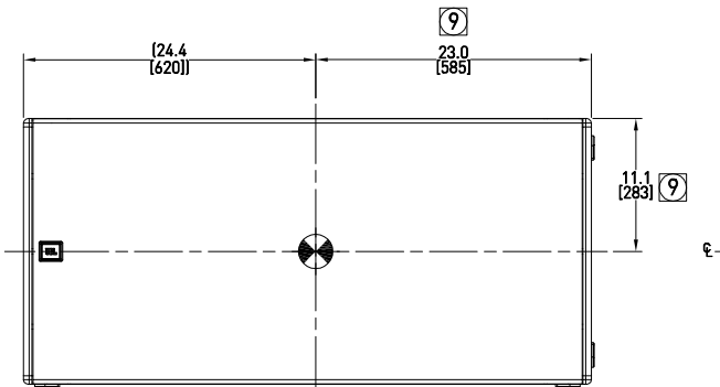
FRONT
